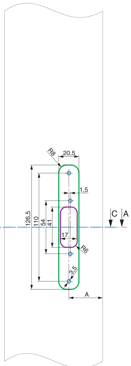
Frame profile (simplified illustration)
