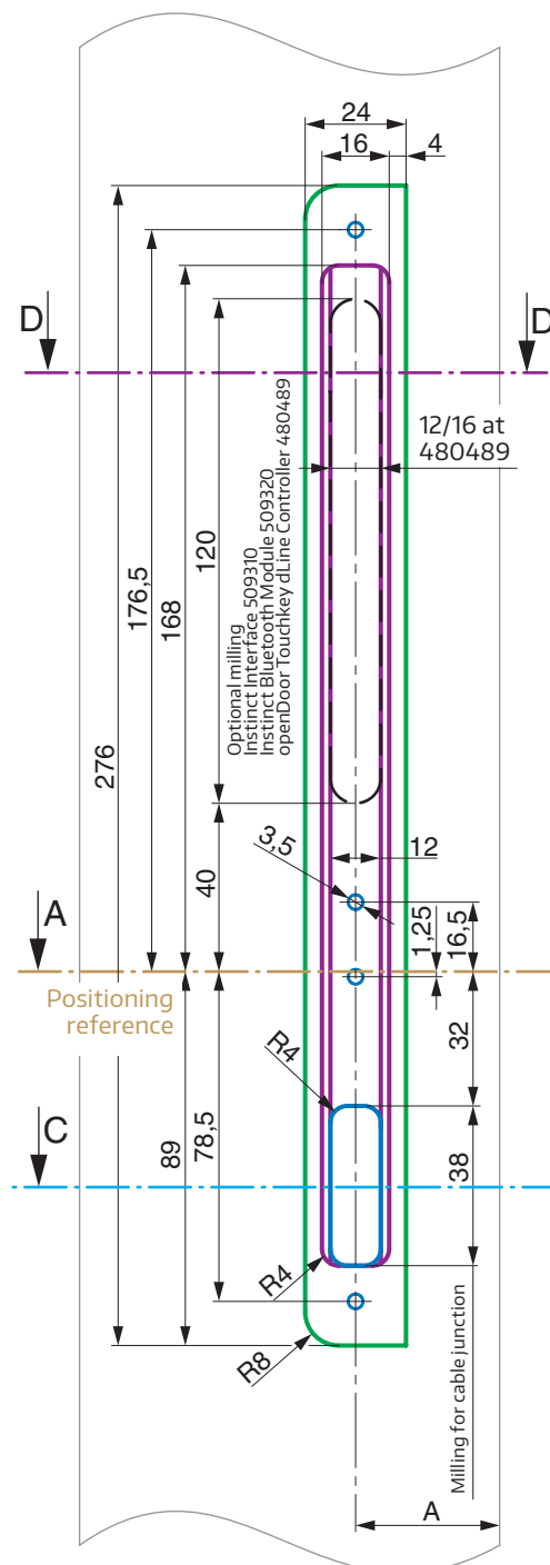
Sash profile (simplified illustration)
